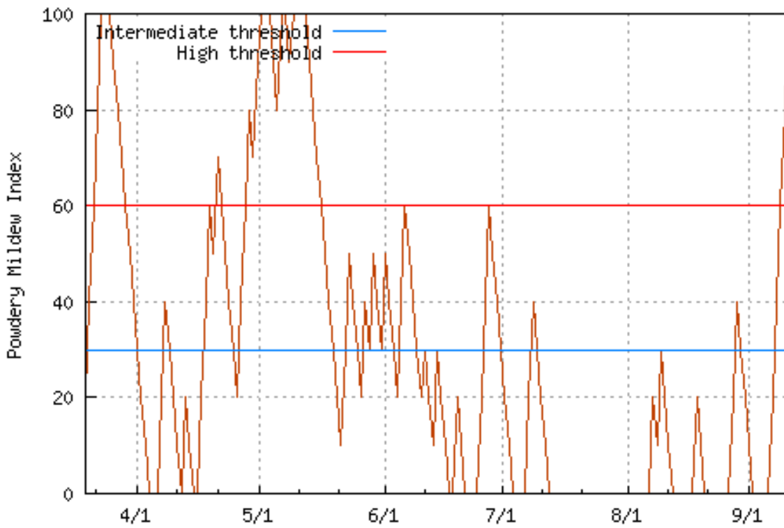
Figure 2. Thomas-Gubler Risk Index data from Apr 1st to Sept 1st. The Red line data points indicate risk index > 60, between blue and red data points indicate risk index data between 30 and 60 and blue data points are values below 30.
